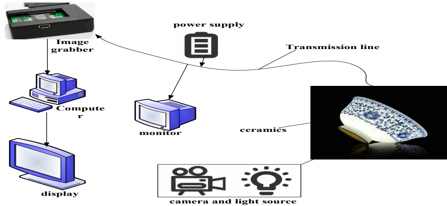
Figure 3: DIP ceramic inspection method
