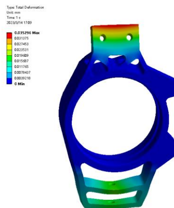
Figure 14: Front Column Total Deformation Diagram.
